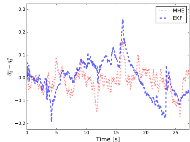
Figure 14: \hat{q}_3^n - q_3^n
