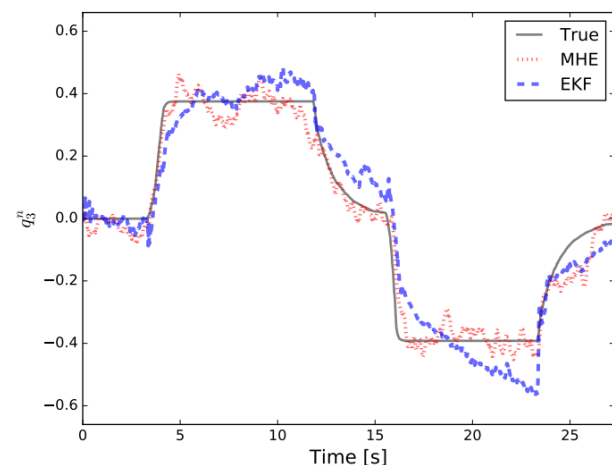
Figure 13: q_3^n
