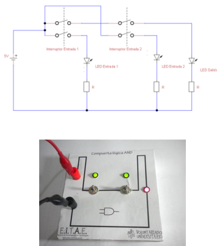
Figura 1: Compuerta AND
